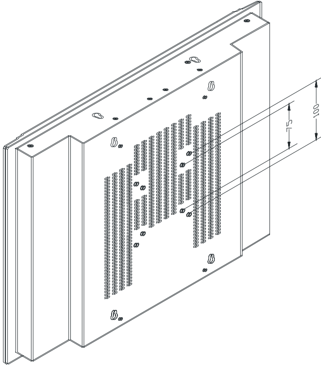
Figure 2.5: Swing-ARM for the FPM-3191G
