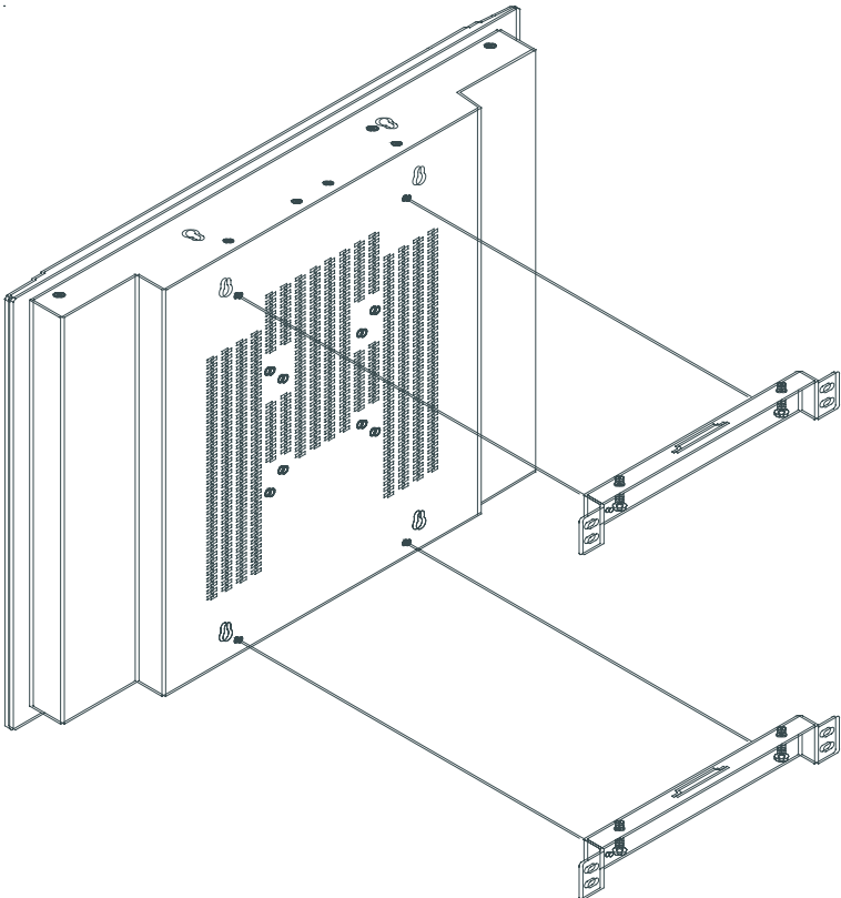
Figure 2.1: Wall Mounting
