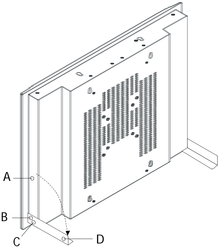
Figure 2.4: Desktop Stand for the FPM-3191G
