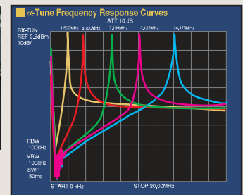
10 dB/Div • 2 MHz/Div
