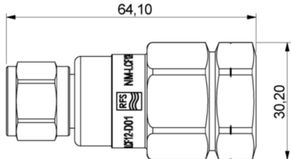
View NM-LCF12-D01_DRW.PNG
