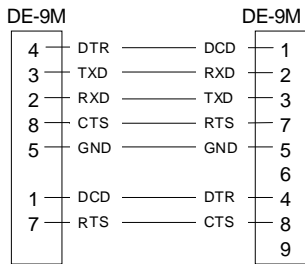
Figure 1-11 DCE Crossover Cable for DOX Mode
