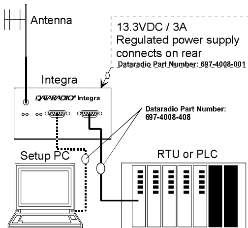
Figure 1-3 Basic Required Connections
