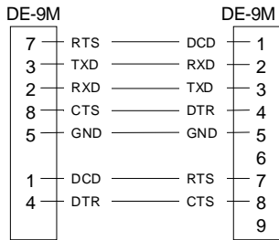
Figure 1-10 DCE Crossover Cable for RTS-CTS mode
