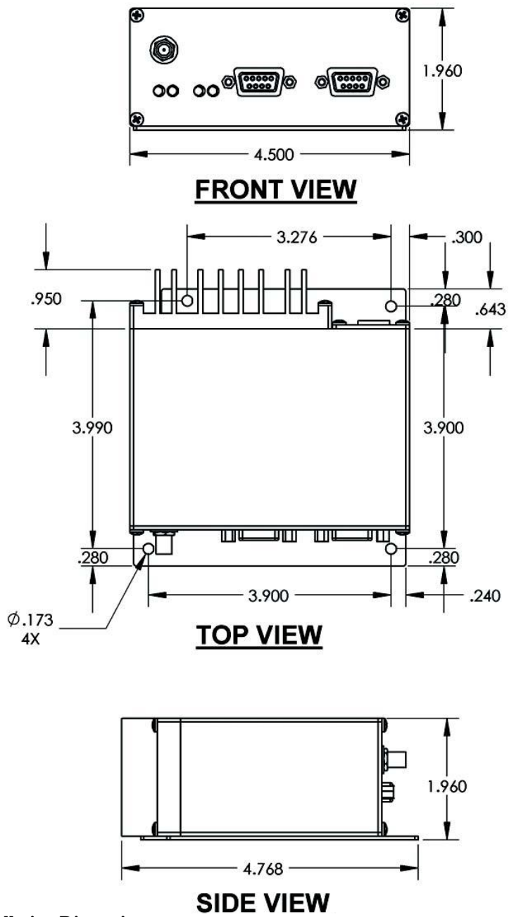
Figure 1-2 Installation Dimensions
