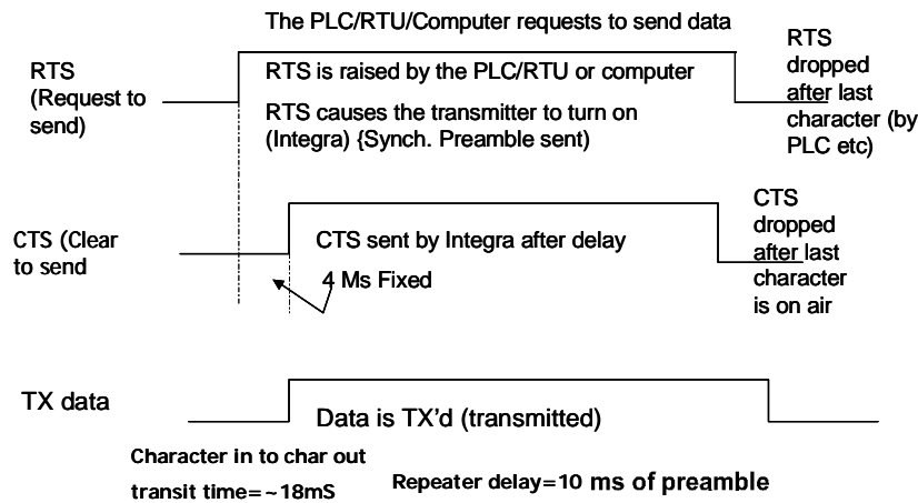
Figure 2-10 Integra-TR Control Signal Timing
