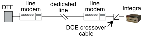
Figure 1-9 Landline (Tail Circuit)
