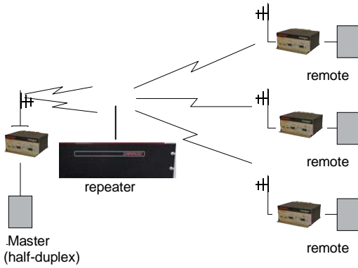
Figure 1-7 Point-Multipoint System (Full-duplex Repeater)
