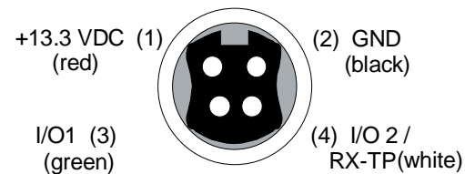
Figure 2-5 I/O Connector
