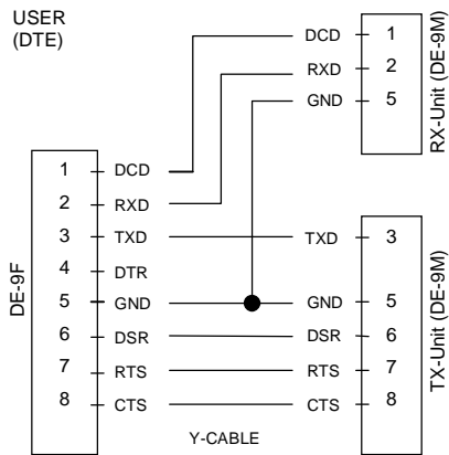
Figure 1-8 Integra-TR Full-duplex Base Station Pinout
