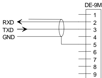
Figure 2-3 3-Wire Interface
