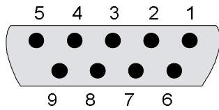
Figure 2-2 COM and Setup Port Connectors Pin Locations
