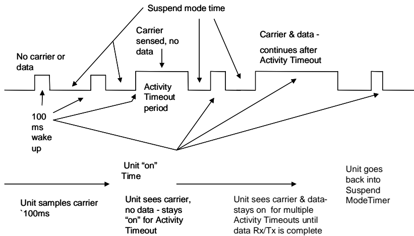
Figure 2-8 Suspend Mode Timing
