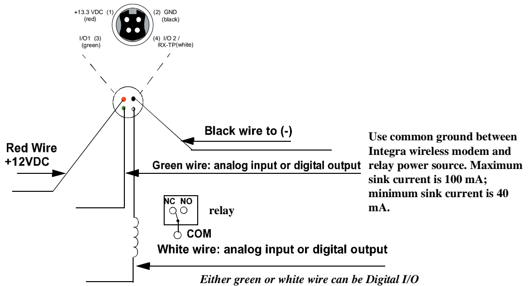
Figure 2-11 Digital I/O Circuit Diagram
