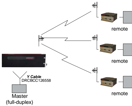
Figure 1-6 Point-Multipoint System (Full-duplex)
