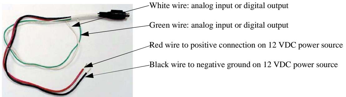
Figure 2-12 Integra Power I/O Cable
